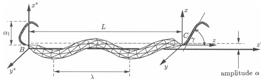
FIGURE 1 Definition of axes and geometrical parameters.
